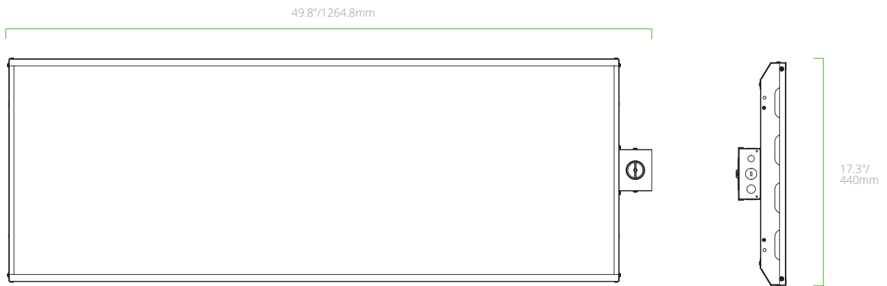
Z10 Receptacle
